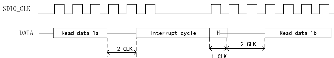
Figure 118 Read Wait Operation through Stop SDIO_CLK
