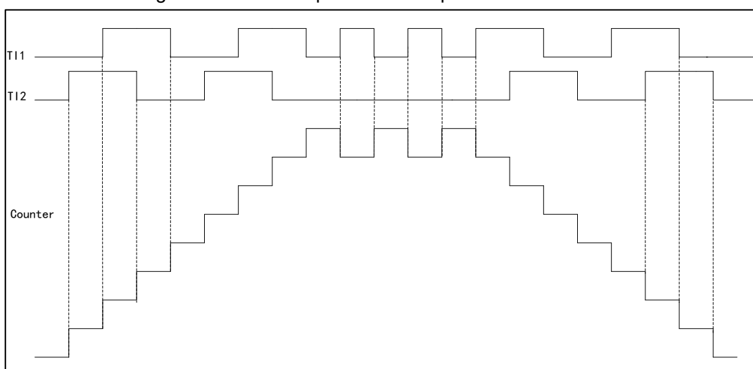
Figure 49 Counter Operation Example in Encoder Mode
