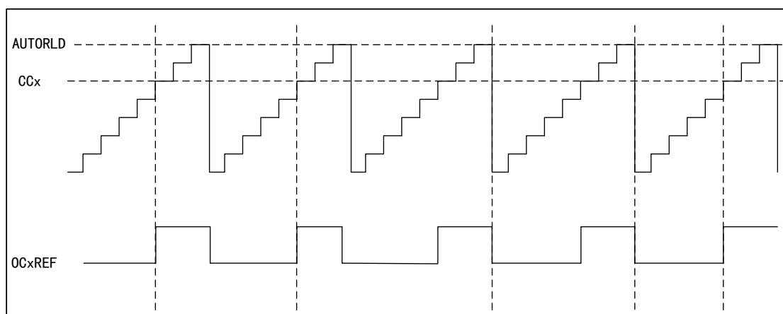
Figure 24 PWM2 Count-up Mode Timing Diagram
