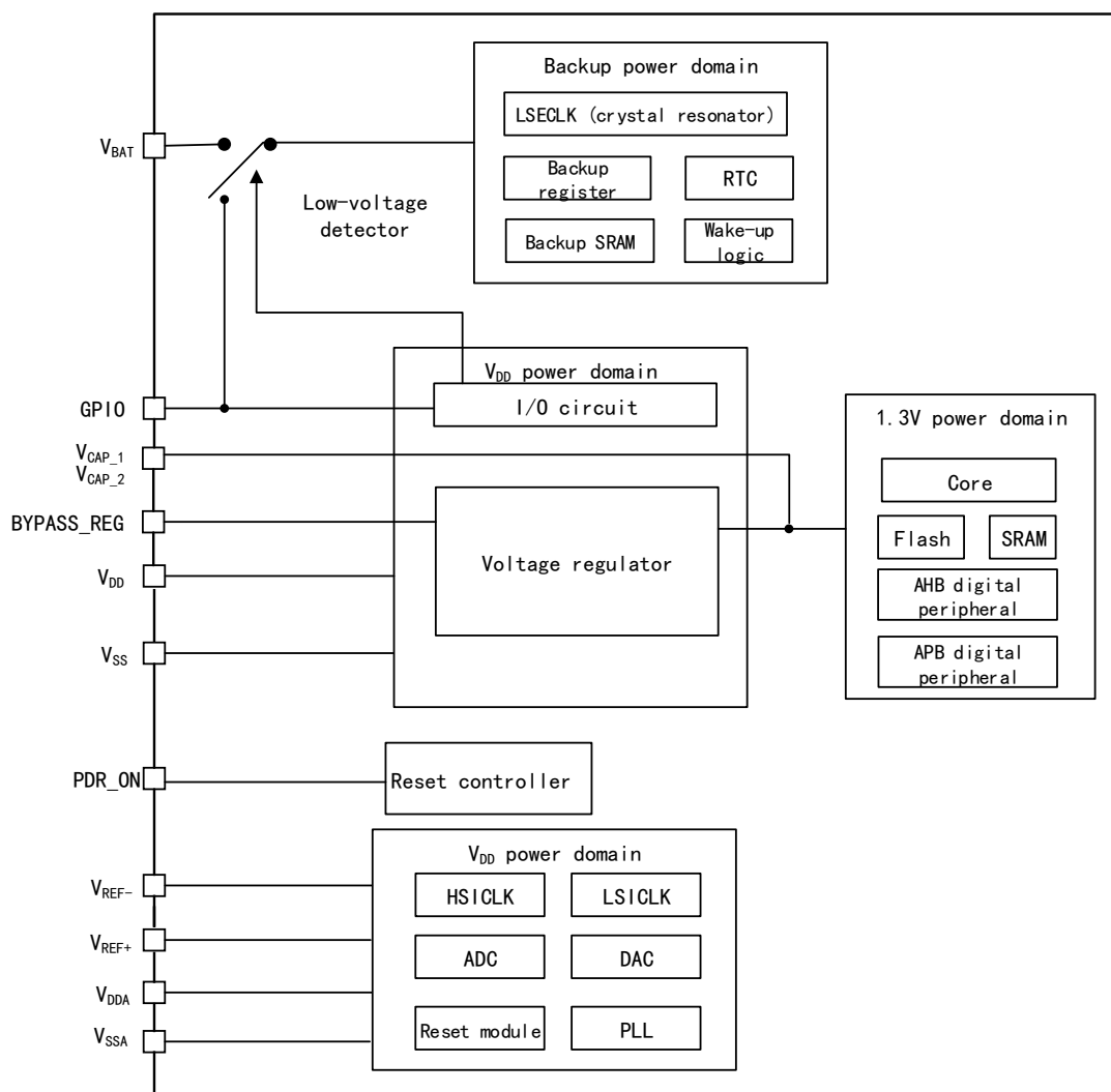
Figure 35 Power Supply Structure Block Diagram
