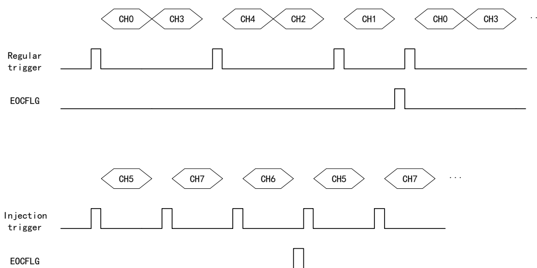
Figure 122 Discontinuous Mode Timing Diagram
