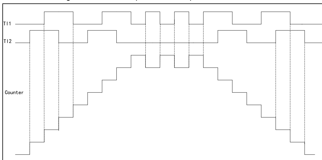
Figure 32 Counter Operation Example in Encoder Mode
