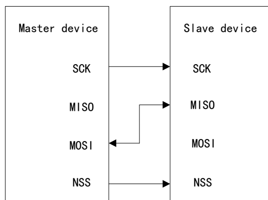
Figure 90 Bidirectional Line Connection
