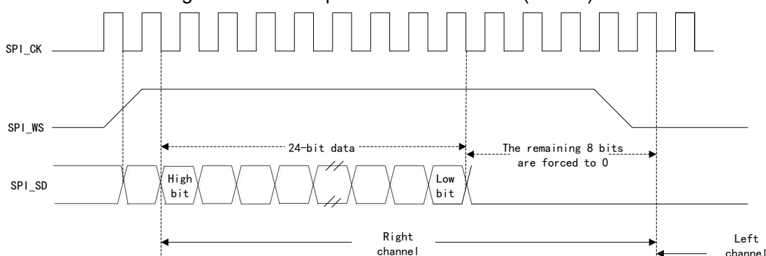
Figure 92 I2S Philips Protocol Waveform (24 bits)
