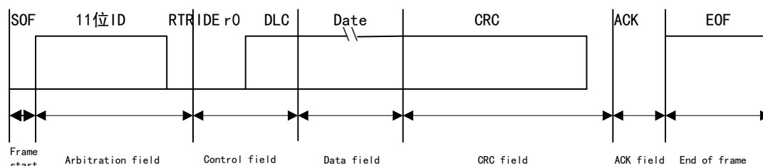
Figure 102 Standard Data Frame
