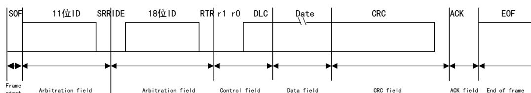
Figure 103 Extended Data Frame
