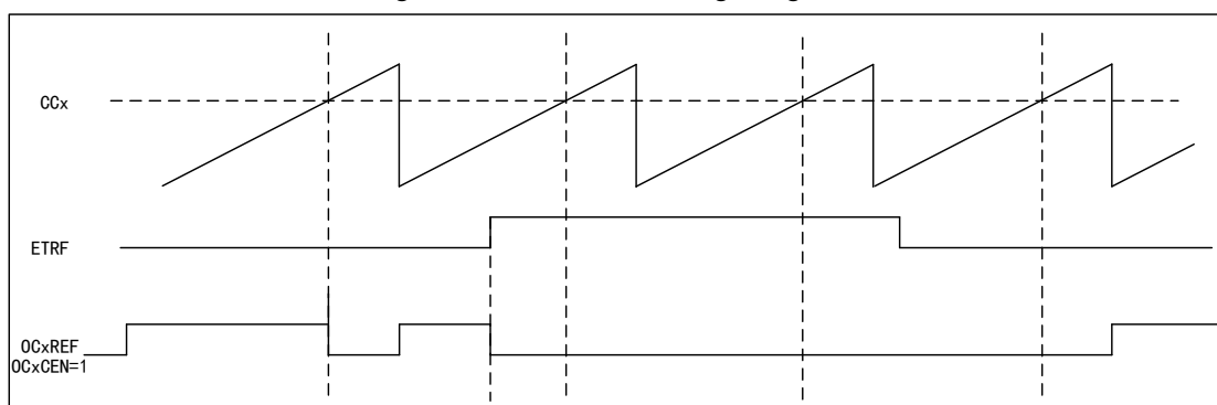
Figure 52 OCxREF Timing Diagram
