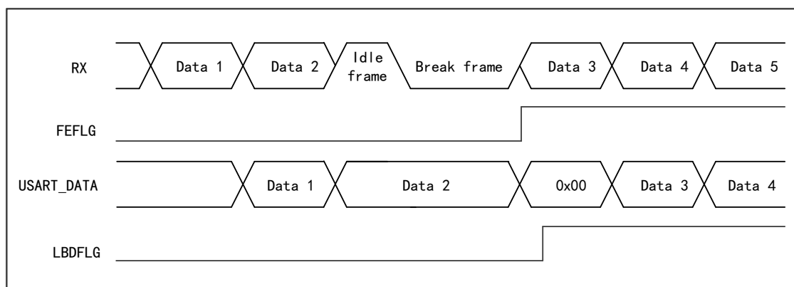
Figure 73 Break Frame Detection in Idle State
