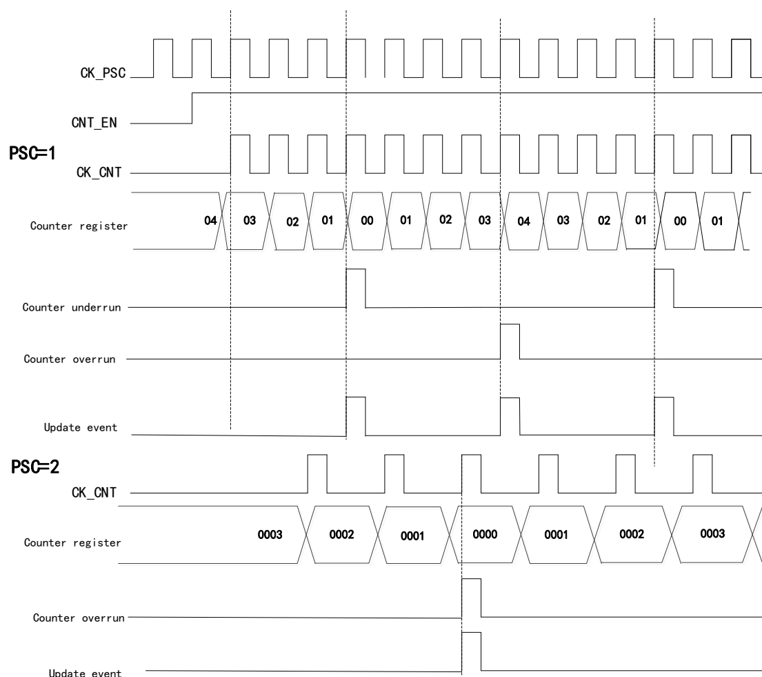
Figure 19 Timing Diagram when Division Factor is 1 or 2 in Center-aligned Mode
