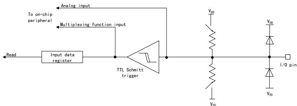
Figure 13 Input Mode Structure
