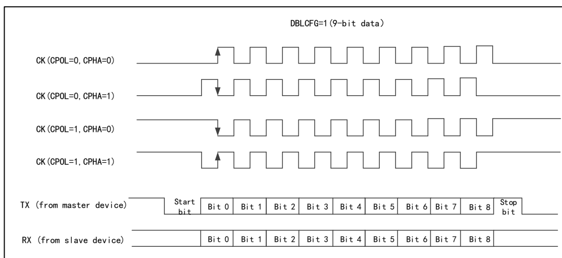
Figure 72 USART Synchronous Transmission Timing Diagram (DBLCFG=1)
