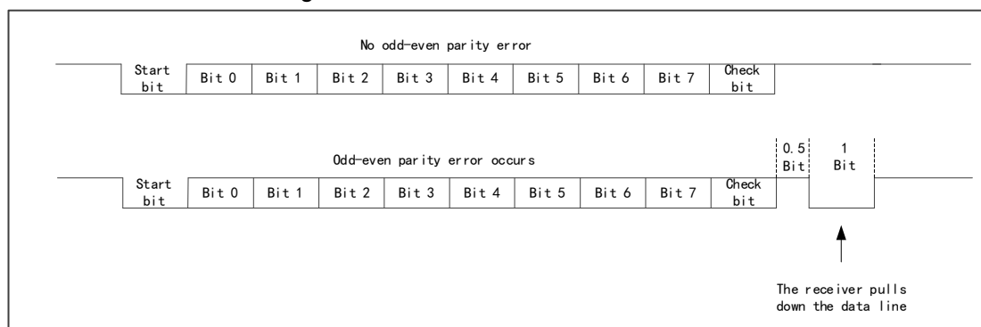
Figure 75 ISO7816-3 Standard Protocol
