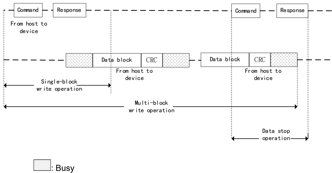
Figure 114 SDIO (Multi-) Data Block Write Operation
