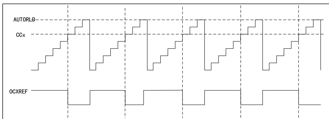
Figure 57 PWM1 Count-up Mode Timing Diagram
