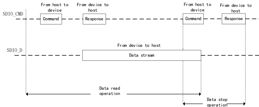
Figure 115 SDIO Data Flow Read Operation
